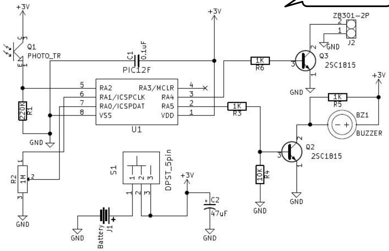
Option:Open Collector Circuit
